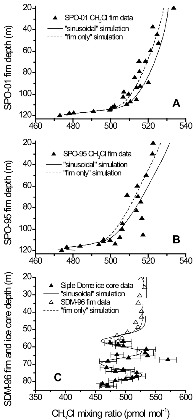
Figure 3. Depth profiles of \text{CH}_3\text{Cl} ice core data and firm air measurements, compared with model simulations based on the “firm only” and “sinusoidal” atmospheric histories shown in Figure 2: (a) South Pole (SPO-01), (b) South Pole (SPO-95), and (c) Siple Dome (ice cores, and SDM-96); the error bars represent the uncertainty in the ice core data. Results from the top 20 m of the firm are omitted because they are subject to seasonal variability. Note that the general trends in all firm data are correctly simulated with the “sinusoidal” history.
