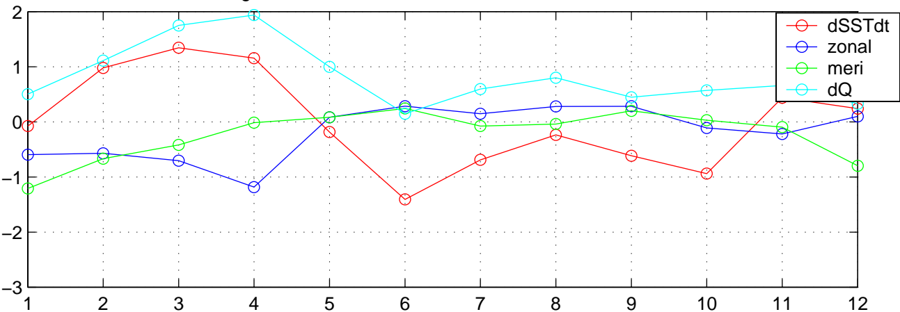
region1 control run, dSSTdt;heat;zonal-adv;meri-adv
