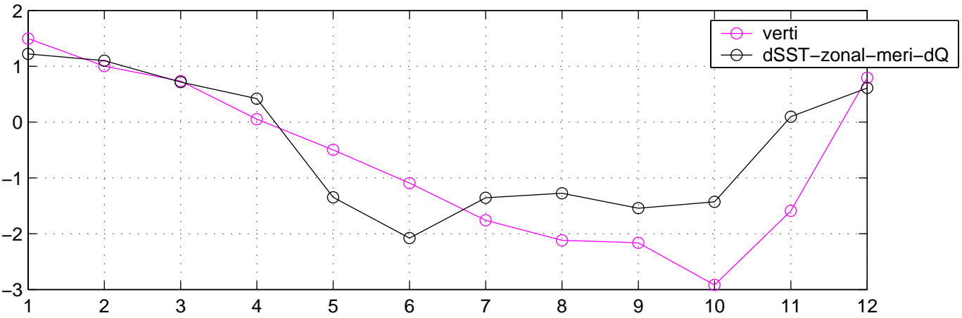
region1 control run, dSST-heat-zonal-meri-vertical-adv
